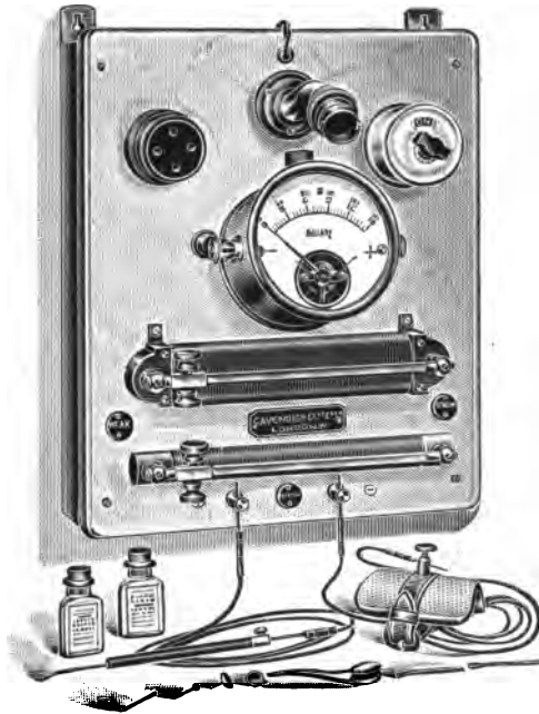
Switchboard for current from a battery.
